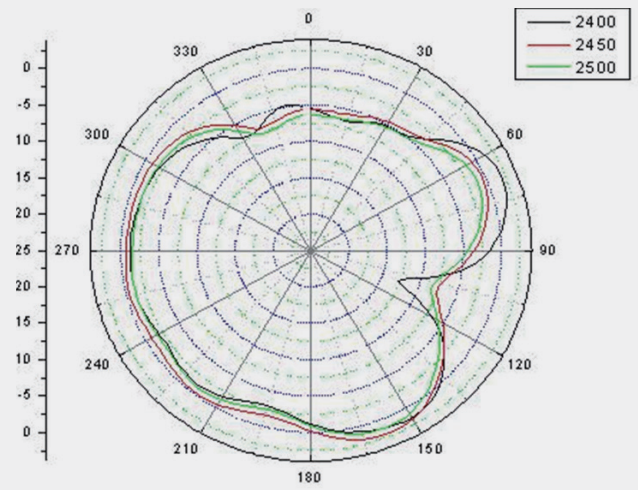
2.4G (PHI=90)
